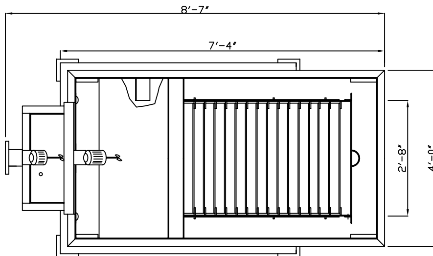
PLAN VIEW
