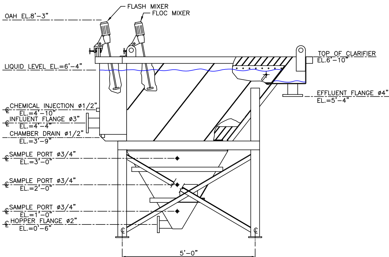
SIDE ELEVATION
